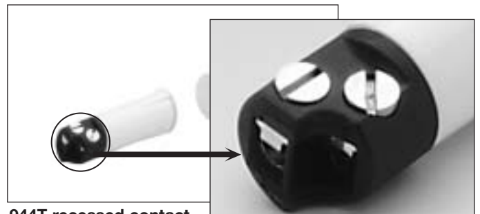
944T recessed contact with staggered terminals
